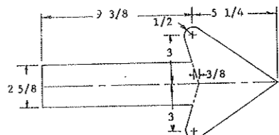
ARROW DETAIL FOR SIGN NOS. G20-5-72 AND G20-6-72
